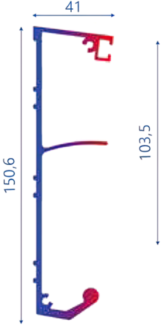
Duvar Dayama Profili 2,394 KG/MT
